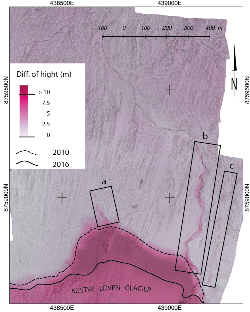
Figure 7: The difference of DEMs between 2010 and 2016 highlights 3 areas where significant mophological changes could be observed. (a) is a main outlet of supra glacial runoff. (b) corresponds to the digging of new channels while (c) is the disappearance of old icing areas. To have a better perception, a transparency was applied to the DoD which is superimposed on the 2016 orthophoto.
