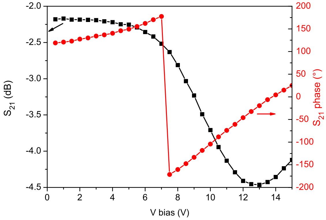
FIG. 5. Response ( S_{21} parameter) of the VCPS versus the control bias voltage. Filled squares, left axis: magnitude in dB. Filled circles, right axis: phase (°).
