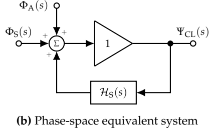
Figure 5. Basic structure of a closed-loop sensor readout system, i.e. an oscillator, together with the random phase contributions of the individual components (a). The use of the phase-space equivalent system (b) simplifies phase noise analysis as phase noise turns into additive noise but requires the determination of the phase-space equivalent transfer function of the sensor \mathcal{H}_S(s) .
