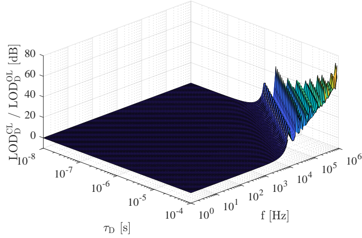
Figure 6. Ratio between the LOD in a closed-loop system (Eq. (43)) and for the LOD in an open-loop system (Eq. (41)) for delay line sensors. Both systems are equal for a wide range of frequencies and delay times, whereas the open-loop system is superior for sensors with large delay times and for the detection of very fast processes.
