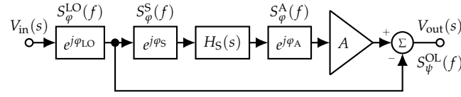
(a) Open-loop system with random phase contributions
