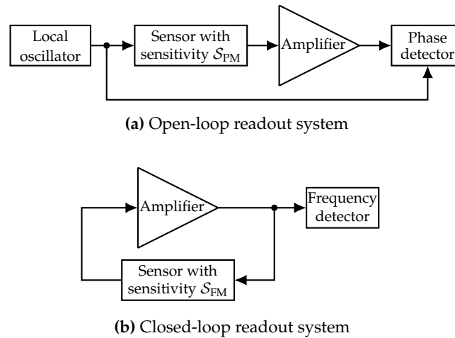
Figure 1. Basic structures of open-loop (a) and closed-loop (b) sensor readout systems. In open-loop systems the signal transceived by the sensor is phase-modulated with a sensitivity S_{PM} whereas the oscillating signal in closed-loop operation is frequency-modulated with a sensitivity S_{FM} .
