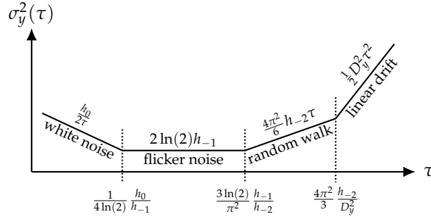
Figure 7. Schematic progression of the Allan variance \sigma_y^2(\tau) as a function of the measurement time \tau for various noise processes and linear drift.
