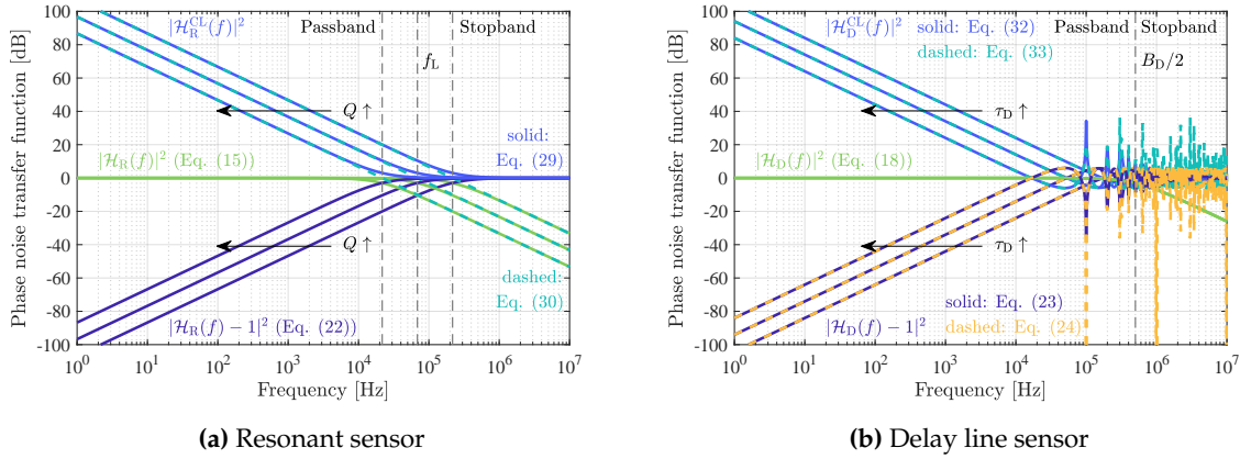
Figure 4. Progression of the calculated phase noise transfer functions in open-loop and closed-loop sensor systems for various quality factors Q of a resonant sensor (a) and various delay times \tau_D of a delay line sensor (b). The chosen sensor parameters are f_R = f_D = 434 MHz, Q = \{1000, 3162, 10000\} , B_D = 1 MHz, and \tau_D = \{1 \mu\text{s}, 3.162 \mu\text{s}, 10 \mu\text{s}\} .
